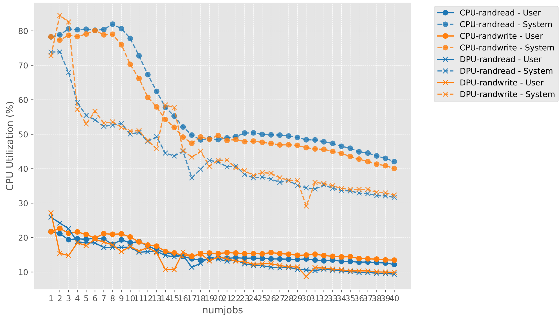
CPU Utilization vs numjobs (CPU vs DPU)
